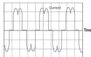
Figure 1 – Non-linear Current
